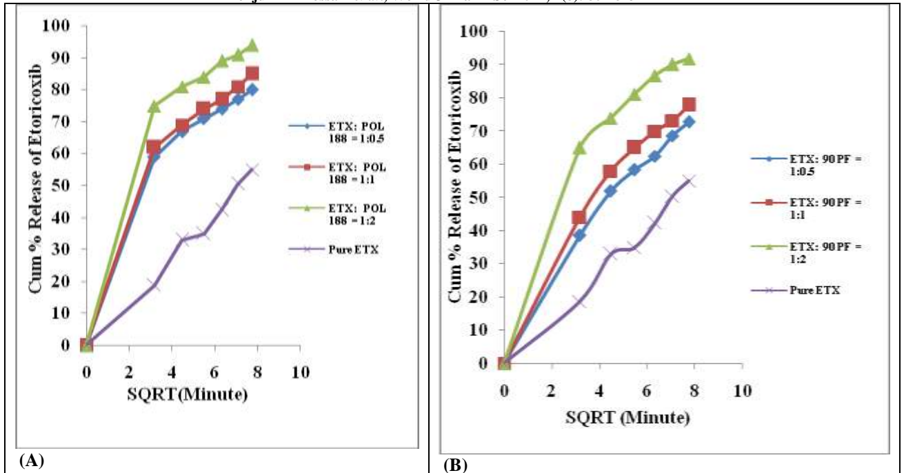
Figure 3. Higuchi release curves of ETX from physical mixtures of ETX with poloxamar 188 (A), kollidon 90F (B) (n = 6).
