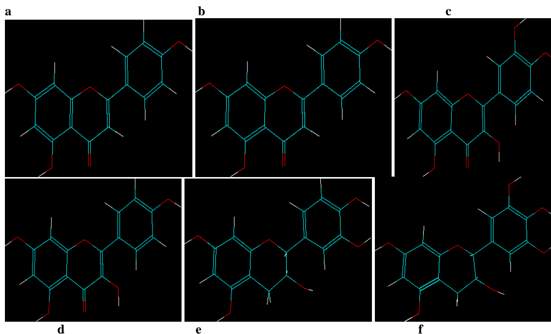
figure 1. 3D cleaned structures of flavonoid derivatives generated by ACD Lab Chemscketch software (a) Apigenin (b) Naringenin (c) Quercetin, (d) Kaempferol (e) Catechin and (f) Gallo catechin
