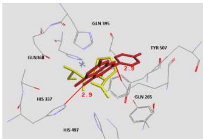
figure 9. Docking of Kaempferol into ACE complexed with co-crystallized ligand captopril. Captopril is seen in yellow and kaempferol in red color. Hydrogen bond interactions are represented in red lines with the distance given in red color
