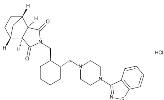
Figure 1: Chemical structure of Lurasidone HCl
