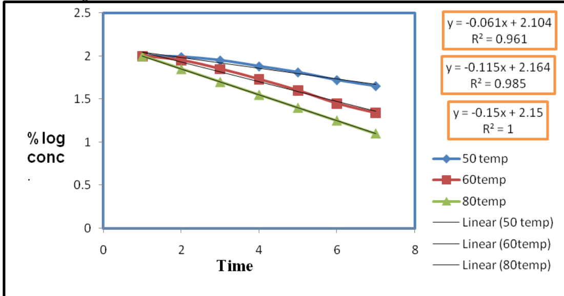
Figure 7: Overlain curve for degradation rate of base at 50 0 c, 60 0 c, 80 0 c
