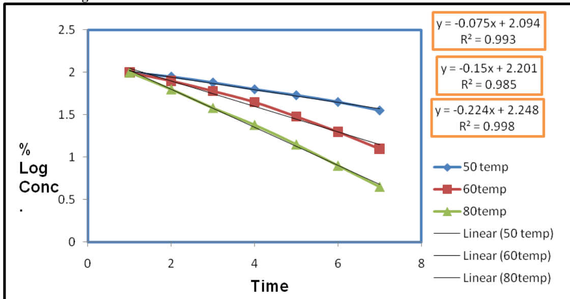
Figure 6: Overlain curve for degradation rate of acid 50 0 c, 60 0 c, 80 0 c
