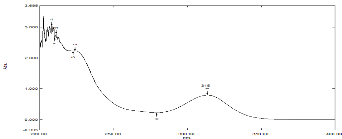
Figure 2: UV spectrum of Lurasidone HCl
